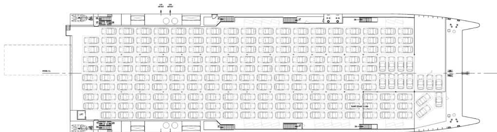
UPPER VEHICLE DECK
