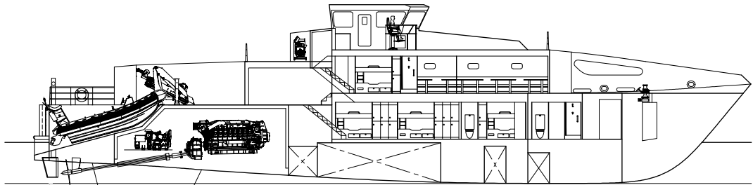
PROFILE @ CENTRELINE
